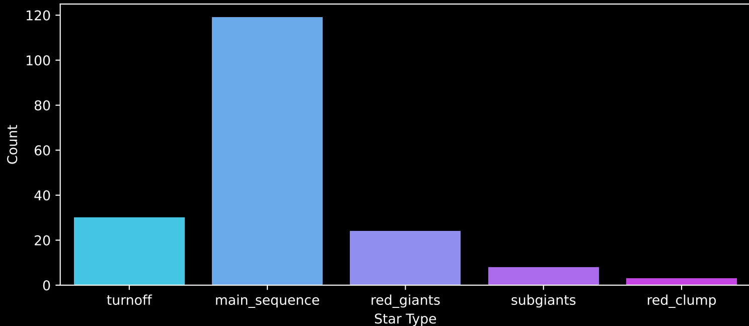
APOGEE DR17 Field: [JHelum6] Count plot of Star Type
