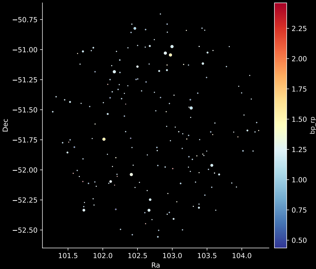
APOGEE DR17 Field: [JHelum6] Stars: 184
