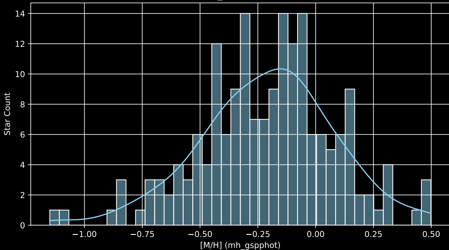
APOGEE DR17 Field: [JHelum6 [M/H] (mh_gspphot) (n= 181)
