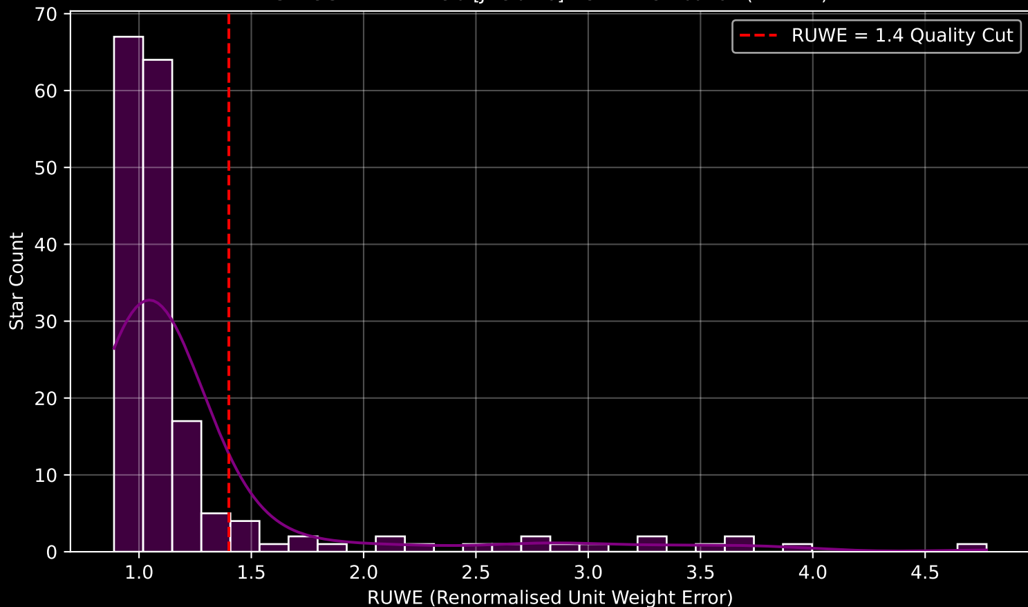
GAPOGEE DR17 Field [JHelium6] RUWE Distribution (n= 177)
