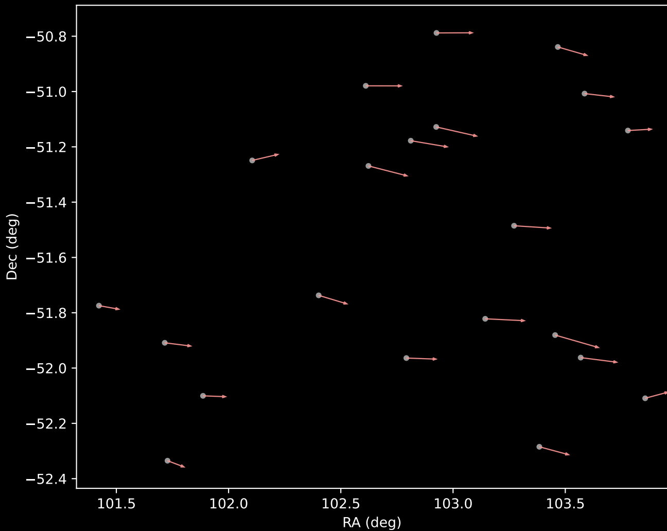
APOGEE DR17 Cluster 7 Proper Motion Vectors (n=21)
