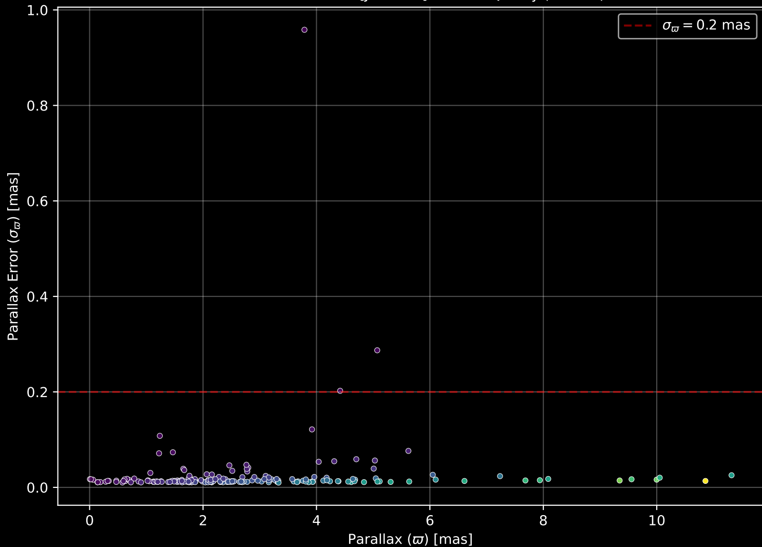
APOGEE DR17 Field: [JHelum6] Parallax Quality (n= 184)
