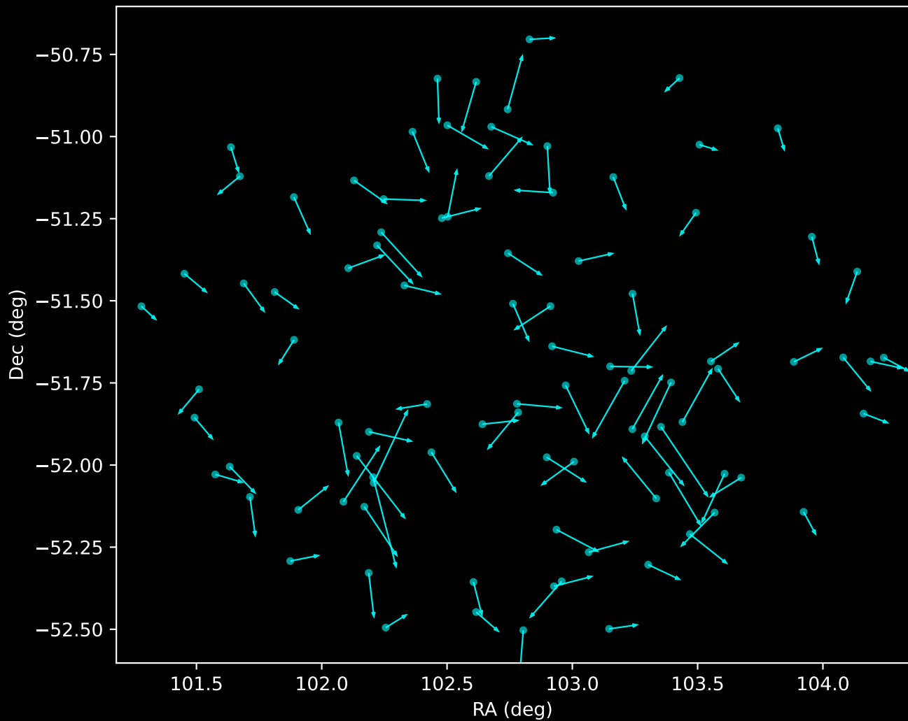
APOGEE DR17 Noise Stream Proper Motion Vectors (n=94)
