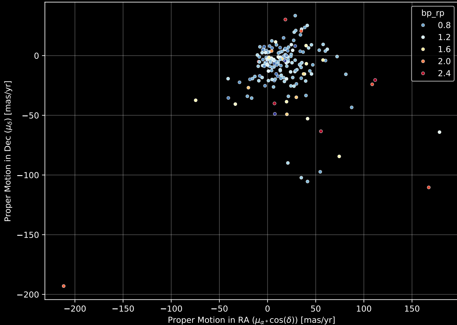
APOGEE DR17 Field: [JHelum6] Proper Motion Diagram (n= 184)
